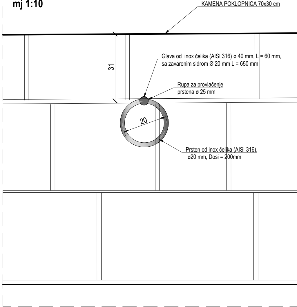
POGLED mj 1:10
